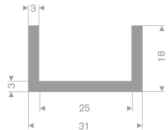
211.00.620GR TPE 70° Shore grey roll length 25 meter
