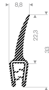
245.00.865 pvc + Sponge rubber clamping range 1-2,5 mm roll length 50 meter
