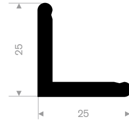
216.52.525 EPDM 60° Shore black roll length 50 meter
