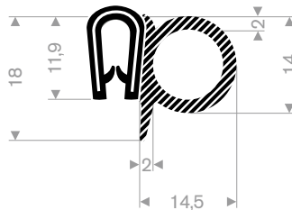
245.00.115 pvc + Sponge rubber clamping range 1,5-3 mm roll length 25 meter
