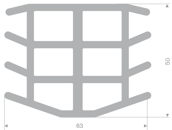
216.06.601 EPDM 70° Shore grey roll length 25 meter
