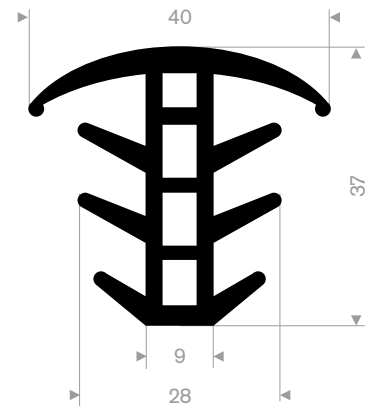
216.05.705 EPDM 70° Shore black roll length 25 meter
