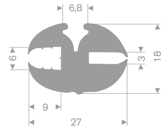
213.00.412GR TPE 70° Shore grey roll length 30 meter
