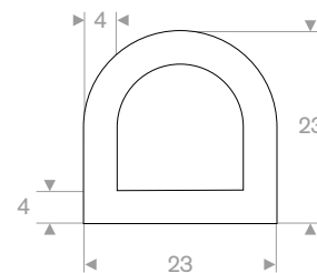
215.00.423W TPE 60° Shore white roll length 25 meter
