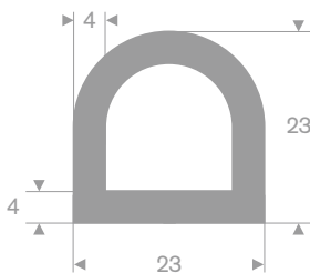
215.00.423GR TPE 60° Shore grey roll length 25 meter
