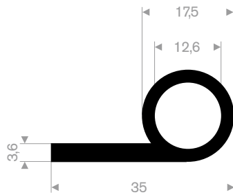
214.00.815 EPDM 70° Shore black roll length 50 meter
