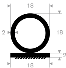
216.00.803 EPDM 90° Shore with adhesive roll length 25 meter
