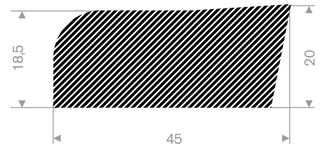
228.14.520 EPDM 15° Shore roll length 25 meter
