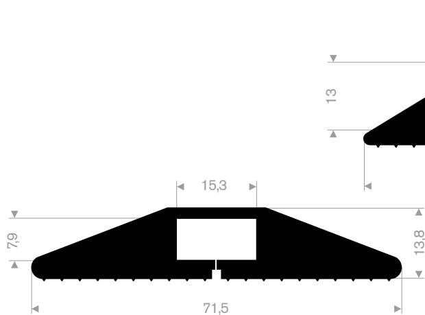
215.00.474 PVC 92° Shore black/yellow roll length 9 meter
