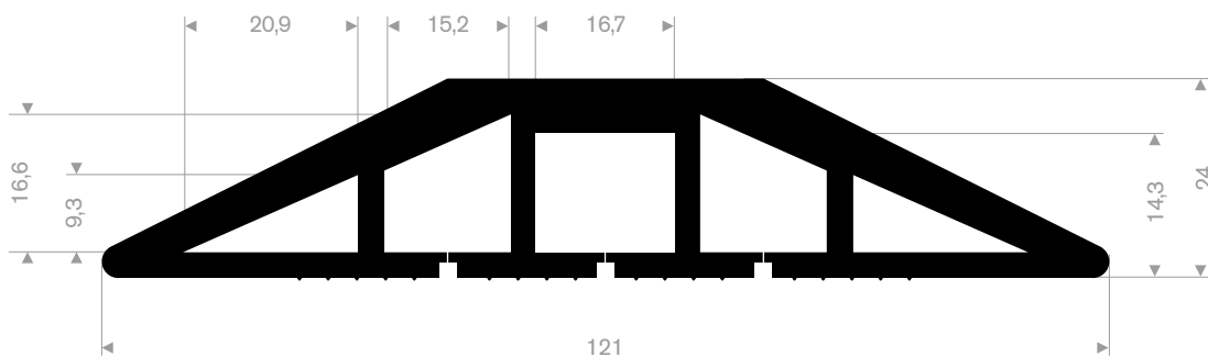
215.00.478 PVC 92° Shore black/yellow roll length 9 meter
