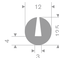
211.04.180GR TPE 70° Shore grey roll length 50 meter
