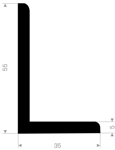
216.55.535 EPDM 60° Shore black roll length 30 meter
