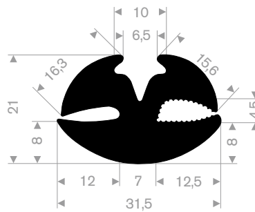
213.00.382 EPDM 70° Shore black roll length 25 meter
